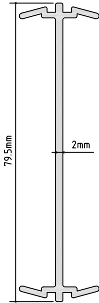
PM 114 100mm FRAME COUPLER (Suits All 100mm PM Sections) A/P: 245.89 mm L/W: 0.609 kg/m
