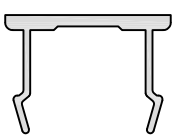
PM 116 POCKET INFILL A/P: 104.23 mm L/W: 0.177 kg/m
