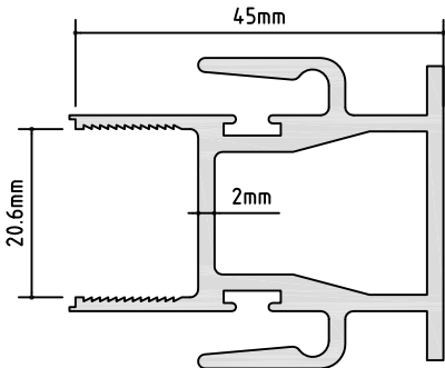
PM789 DOUBLE INTERLOCK A/P: 320.15 mm L/W: 1.006 kg/m
