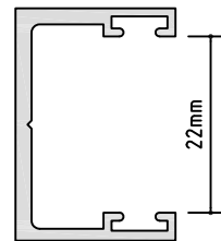
PM740 SCREEN DOOR CHANNEL A/P: 161.54 mm L/W: 0.336 kg/m
