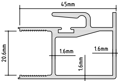
PM767 DG STANDARD INTERLOCK A/P: 252.38 mm L/W: 0.787 kg/m
