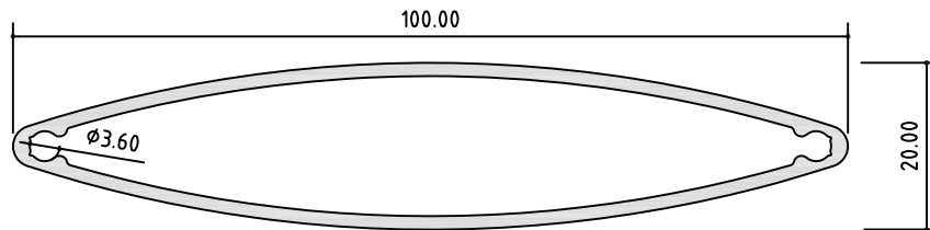
LVR50837 LOUVRE BLADE A/P: 208.85 mm L/W: 0.887 kg/m
