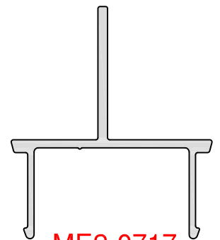
ME2-0717 50mm SASH ADAPTOR A/P: 194.02 mm L/W: 0.402 kg/m
