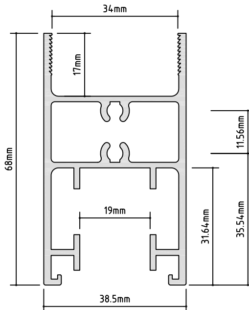
PM 807 DG ONE PART RAIL A/P: 424.97 mm L/W: 1.355 kg/m
