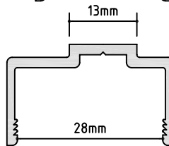
PM 488 24mm GLAZING ADAPTOR A/P: 142.32 mm L/W: 0.328 kg/m
