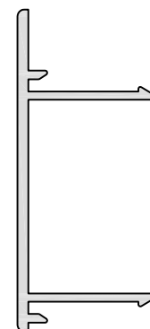
PM 695 INTERLOCK STILE INLAY A/P: 182.86 mm L/W: 0.345 kg/m
