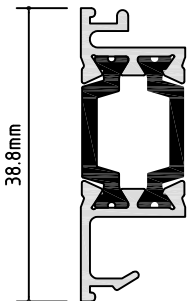
PATH 143 FRAME POCKET FILLER A/P: 133.26 mm L/W: 0.295kg/m
