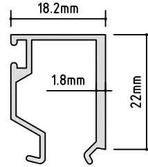
PM 054 Bulb Seal
