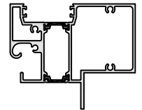
PATH 110 100mm 50mm TH AWNING HEAD / TRANSOM Pg - 98
