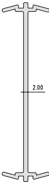
PM 114 100mm FRAME COUPLER A/P: 245.89 L/W: 0.609 kg/m
