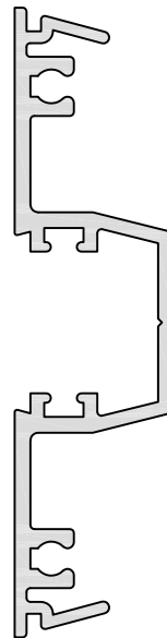
PMA5987 PM 110 GLAZING ADAPTOR A/P: 345.65 mm L/W: 0.865 kg/m
