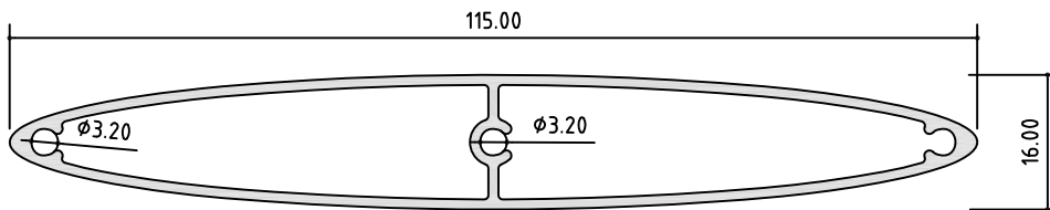
LVR3214 LOUVRE BLADE A/P: 236.40 mm L/W: 0.849 kg/m
