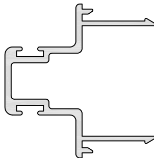
PM 693 MALE MEETING STILE ADAPTOR A/P: 253.74 mm L/W: 0.519 kg/m
