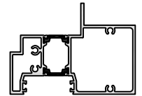
PATH 112 100mm 50mm TH AWNING SILL / TRANSOM Pg - 98
