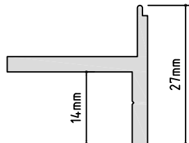
PM 448 TRACK SUPPORT A/P: 108.82 mm L/W: 0.385 kg/m
