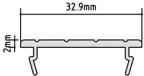
PM 416 TREAD THRESHOLD A/P: 104.10 mm L/W: 0.218 kg/m
