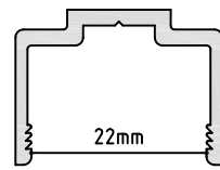
PM 487 18mm GLAZING ADAPTOR A/P: 130.32 mm L/W: 0.296 kg/m
