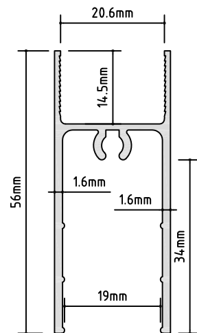
PM774 DG 56mm L/W RAIL A/P: 306.00 mm L/W: 0.612 kg/m
