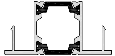
PATH 158 TB TRACK INFILL A/P: 197.40 mm L/W: 0.518 kg/m
