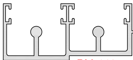
PM 446 DOUBLE TRACK ADAPTOR A/P: 362.64 mm L/W: 0.809 kg/m
