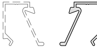
ME2-20237 C.O.C TRANSOM A/P: 466.38 mm L/W: 1.279 kg/m
