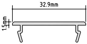
PM 405 PLAIN TRACK INFILL A/P: 101.34 mm L/W: 0.179 kg/m
