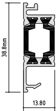
PATH 143 FRAME POCKET FILLER A/P: 133.26 mm L/W: 0.295kg/m
