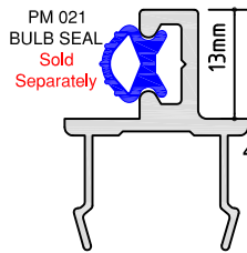
PM 116 POCKET INFILL A/P: 104.23 mm L/W: 0.177 kg/m
