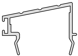
PM 440 RAMPED THRESHOLD A/P: 172.31 mm L/W: 0.298 kg/m
