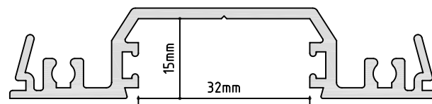
PM 236 GLAZING ADAPTOR A/P: 330.53 mm L/W: 0.848 kg/m
