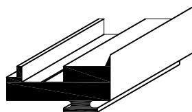
PM067 INTERLOCK ANTI LIFT BLOCK
