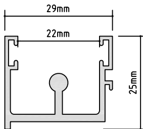
PM 447 SINGLE TRACK ADAPTOR A/P: 204.15 mm L/W: 0.438 kg/m
