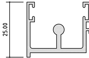
PM 447 SINGLE SILL TRACK ADAPTOR A/P: 204.15 mm L/W: 0.436 kg/m
