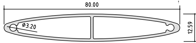
PM622 LOUVRE BLADE A/P: 166.06 mm L/W: 0.587 kg/m
