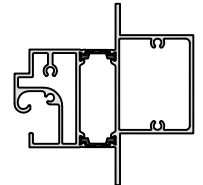
PATH 111 100mm 50mm TH AWNING TRANSOM Pg - 98
