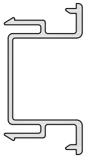
PM 694 FEMALE MEETING STILE ADAPTOR A/P: 198.04 mm L/W: 0.328 kg/m
