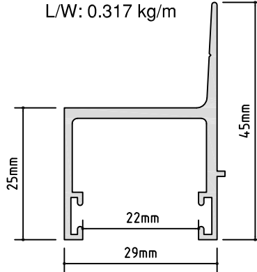
PM 445 SINGLE HEAD TRACK ADAPTOR A/P: 221.01 mm L/W: 0.471 kg/m
