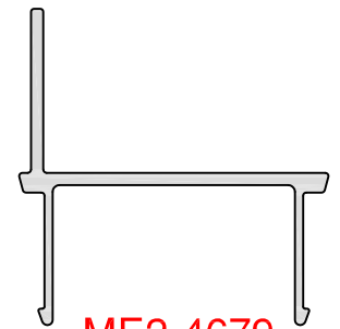
ME2-4679 35mm SASH ADAPTOR A/P: 184.13 mm L/W: 0.343 kg/m
