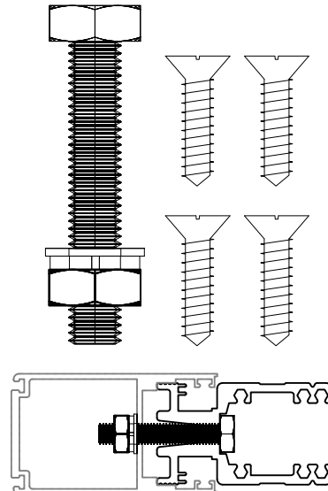
PM 829 SPIGOT SET
