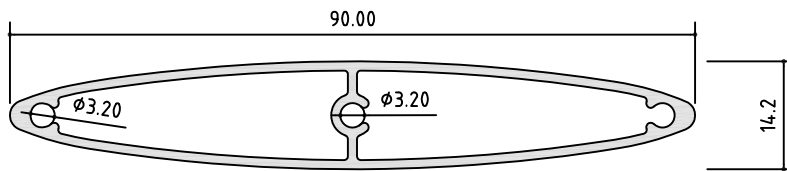
LVR3213 LOUVRE BLADE A/P: 186.51 mm L/W: 0.687 kg/m
