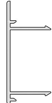
PM 695 INTERLOCK STILE INLAY A/P: 182.86 mm L/W: 0.345 kg/m
