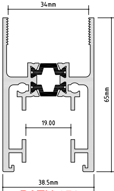
PATH 156 S-DOOR STANDARD RAIL A/P: 485.53 mm L/W: 1.411 kg/m
