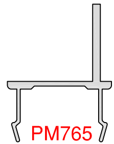
AWNING SASH ADAPTOR A/P: 157.98 mm L/W: 0.301 kg/m
