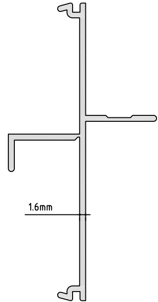
PM 115 100mm REVEAL ADAPTOR A/P: 294.26 mm L/W: 0.613 kg/m
