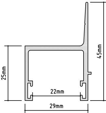
PM 445 SINGLE HEAD TRACK ADAPTOR A/P: 221.01 mm L/W: 0.473 kg/m
